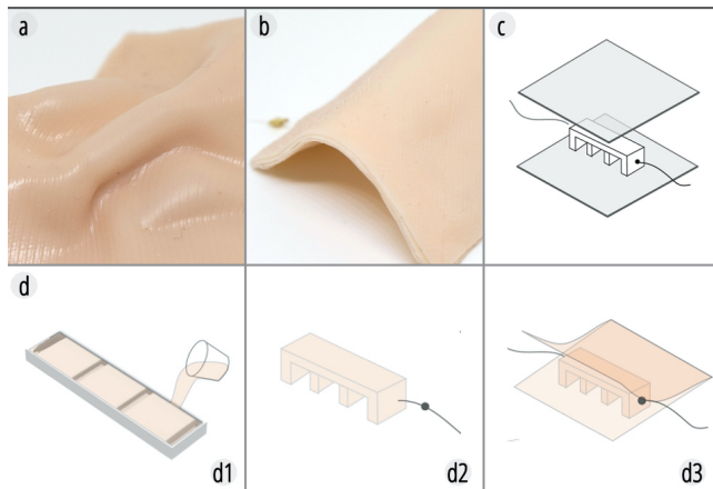
Figure 7: Sample (a-b), exploded view (c), and fabrication process (d) of transformative wrinkles and cheekbone.
