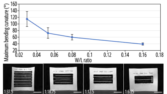
Figure 10. Maximum bending angle changes according to the W/L ratio of the actuator. (Scale bar: 10mm)
